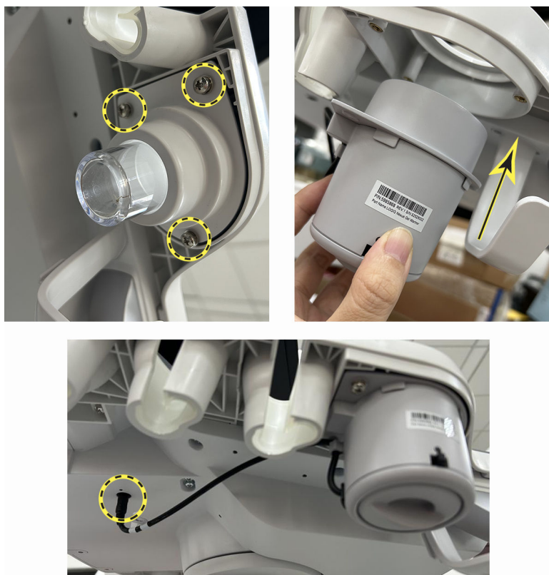
Figure 4-32 Install Gel Warmer
