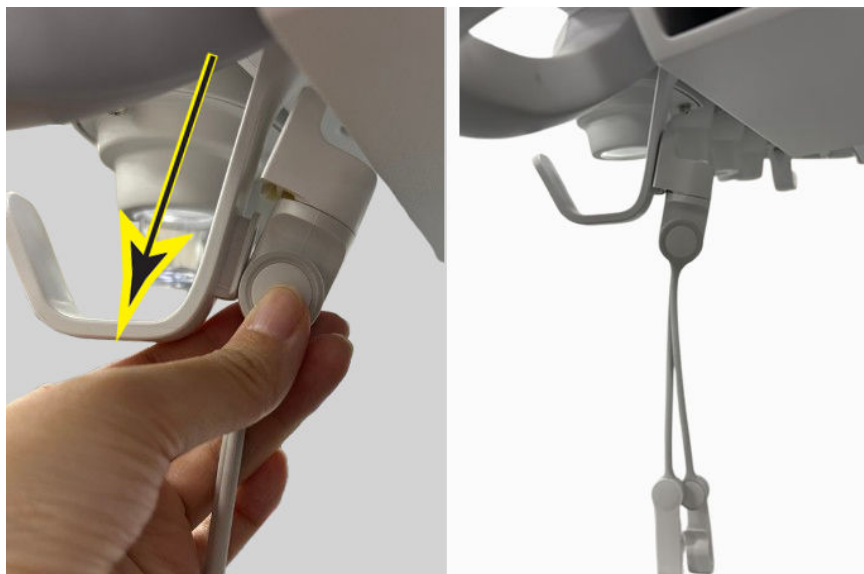
Figure 4-29 Install the Elastic Cable Hook
