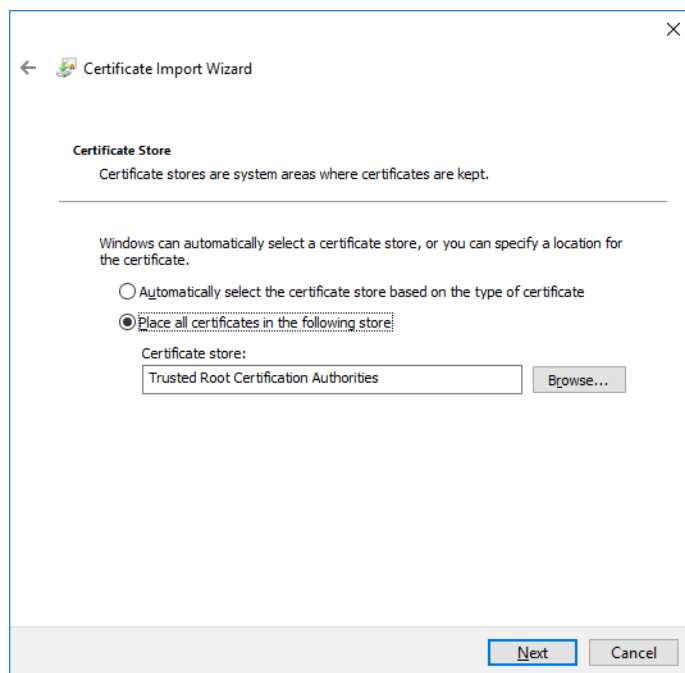
Figure 5-31 Certificate Store
