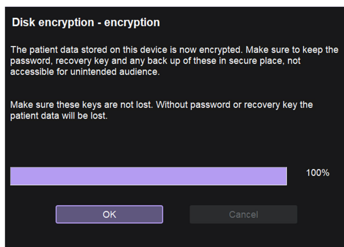
Figure 5-76 Encryption complete
