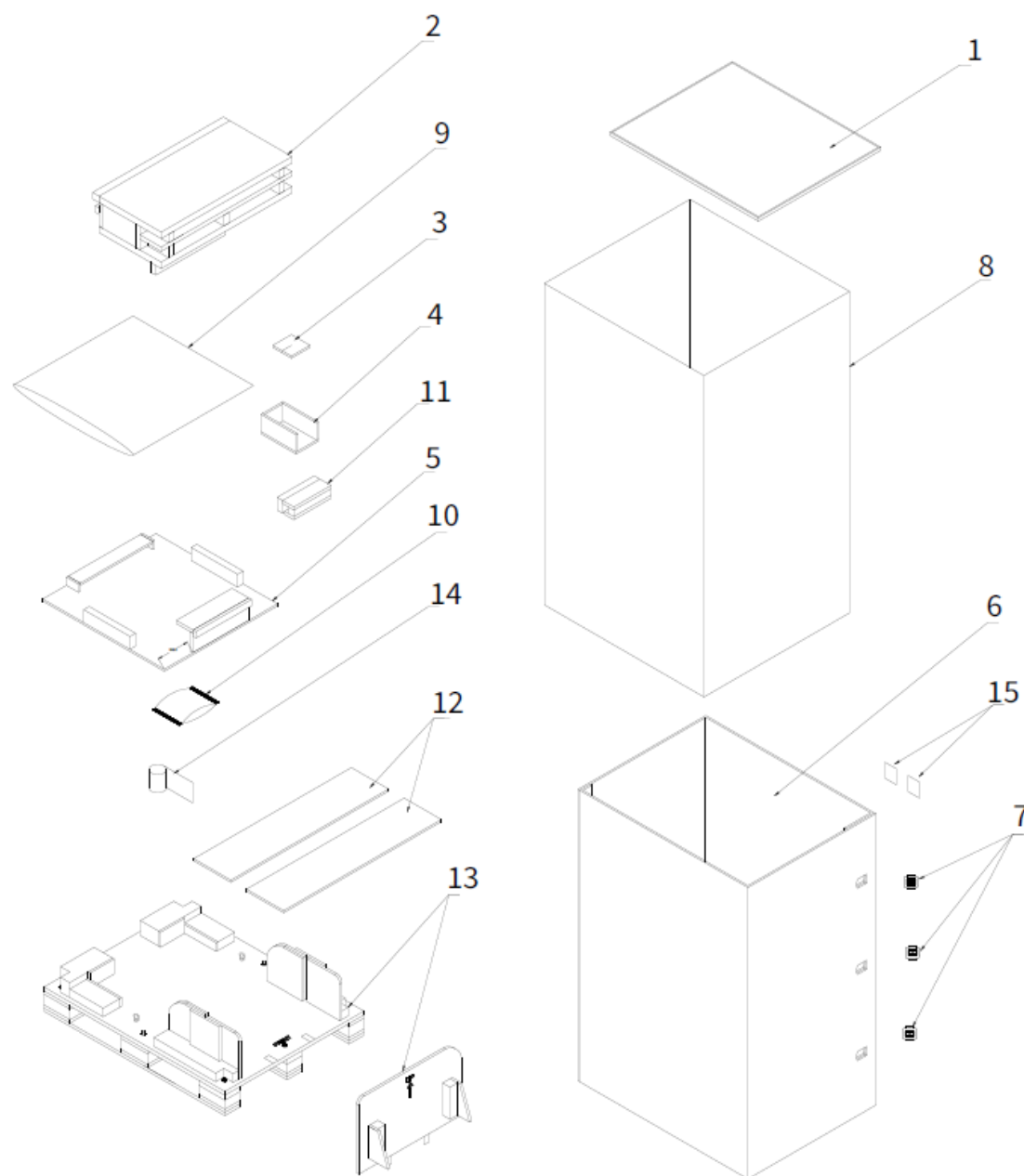
Figure 4-17 Packaging structure
