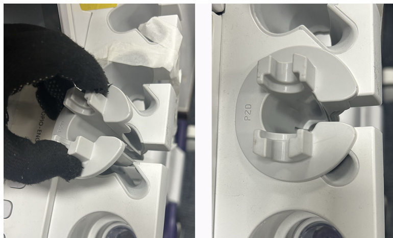
Figure 4-34 Install Ergonomic P2D Probe Holder
