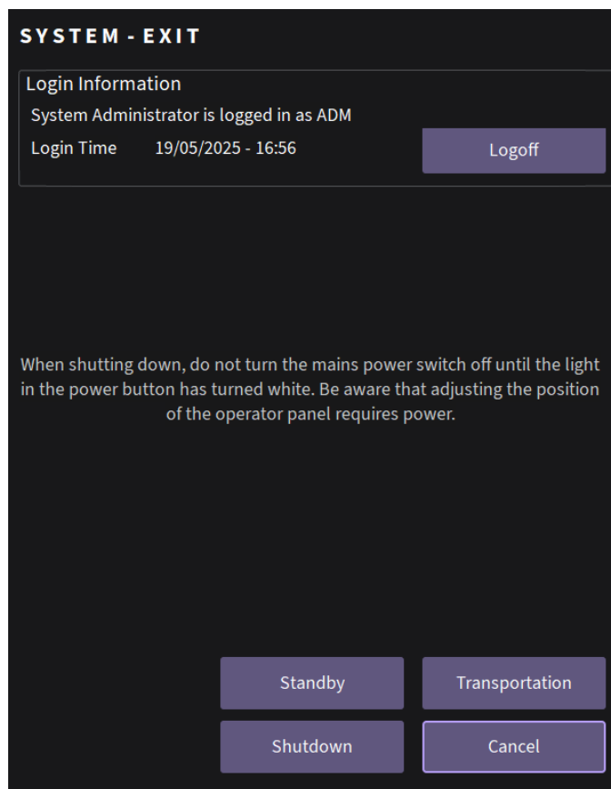
Figure 4-9 Select Shutdown
