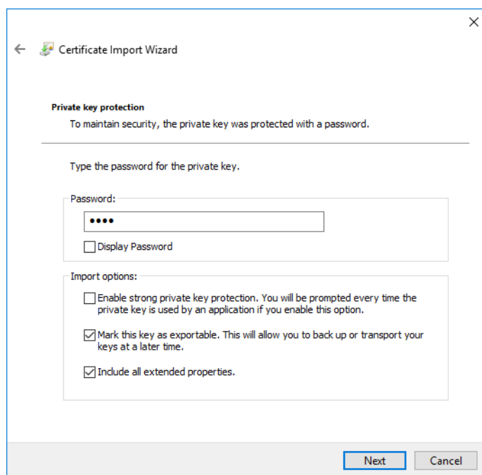
Figure 5-30 Enter Password
