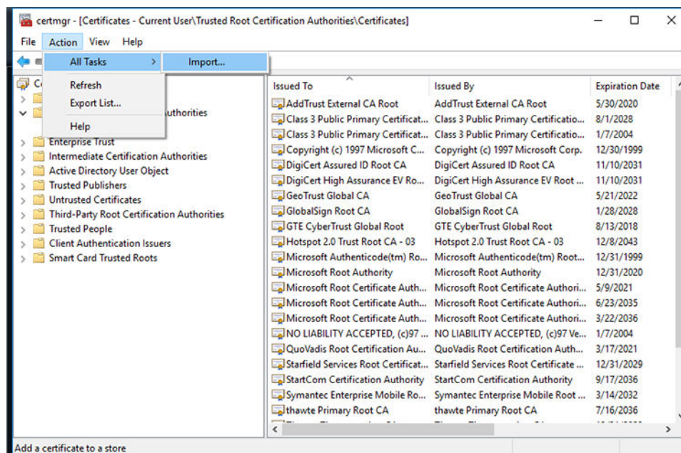
Figure 5-27 Import certificate
