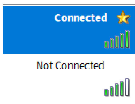
Figure 5-15 Connection Established
