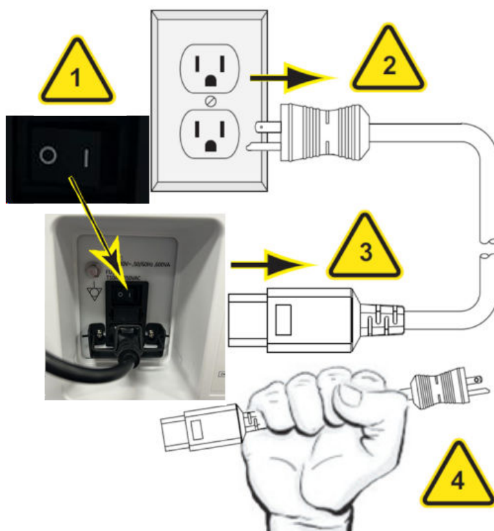
Figure 4-10 Disconnect Power Cord
